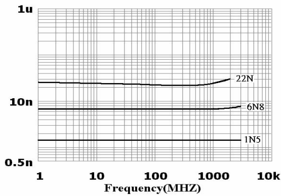
PFCI 1608(0603) TYPE
