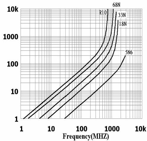
PFCI 1608(0603) TYPE
