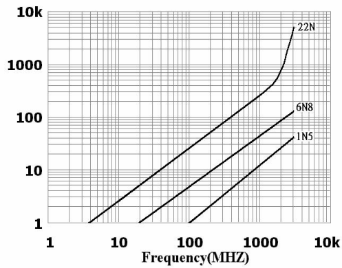
PFCI 0603(0201) TYPE
