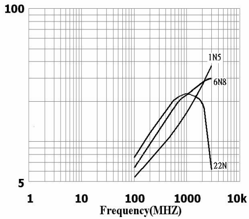
PFCI 1608(0603) TYPE
