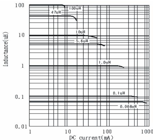
PFFI 3225(1210) TYPE
