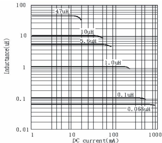
PFFI 3216(1206) TYPE
